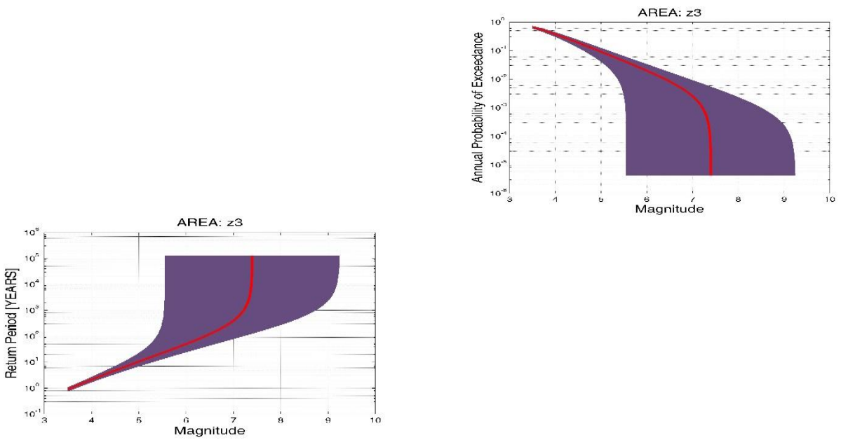
Figure 5. The frequency diagram and return period for Zone 3.
