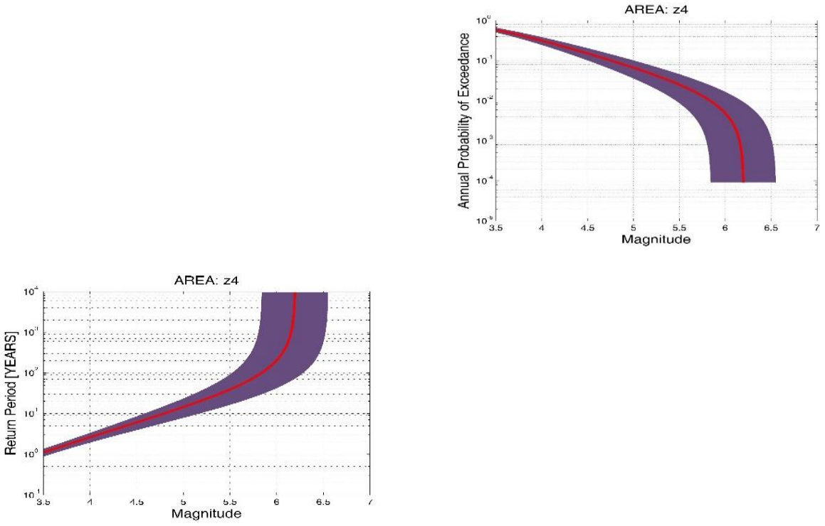
Figure 6. The frequency diagram and return period for Zone 4.
