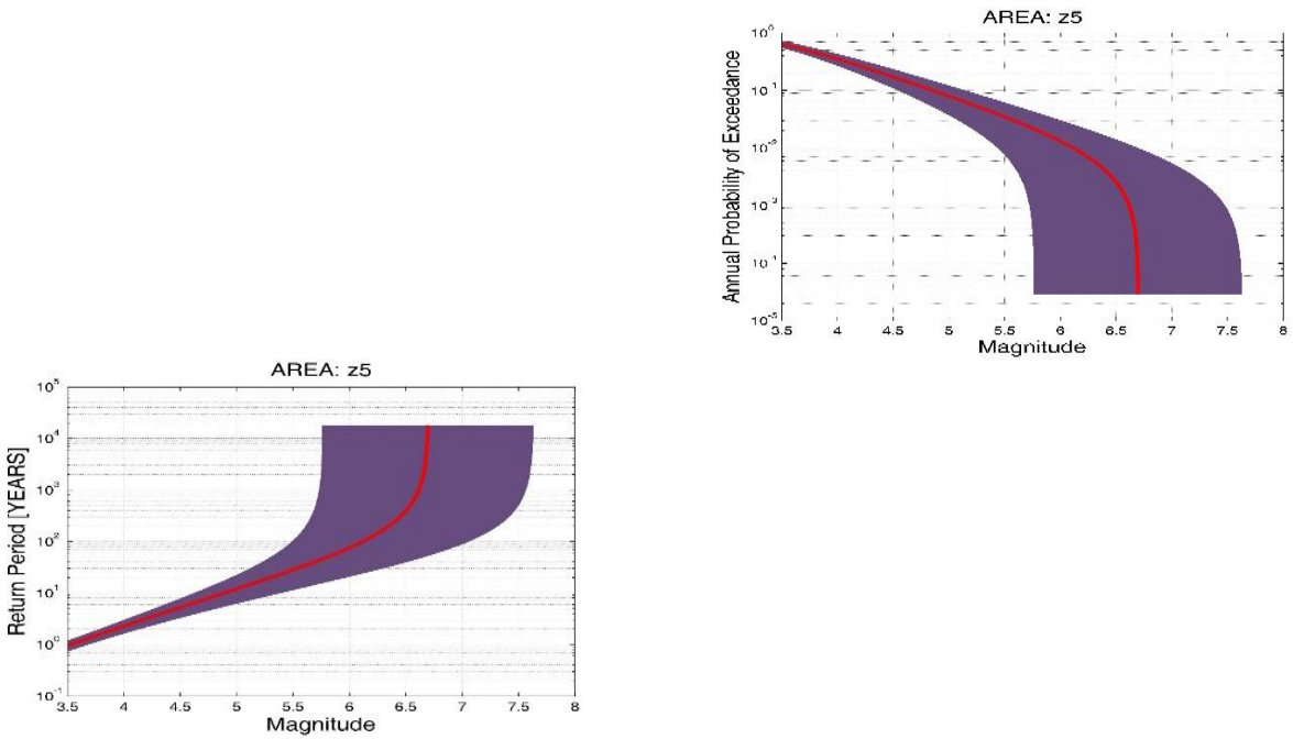
Figure 7. The frequency diagram and return period for Zone 5.
