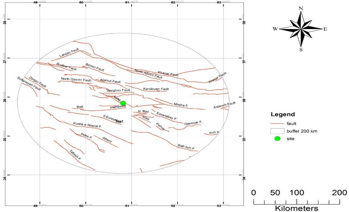
Figure 1. Major faults within a radius of 200 km from the study area.
