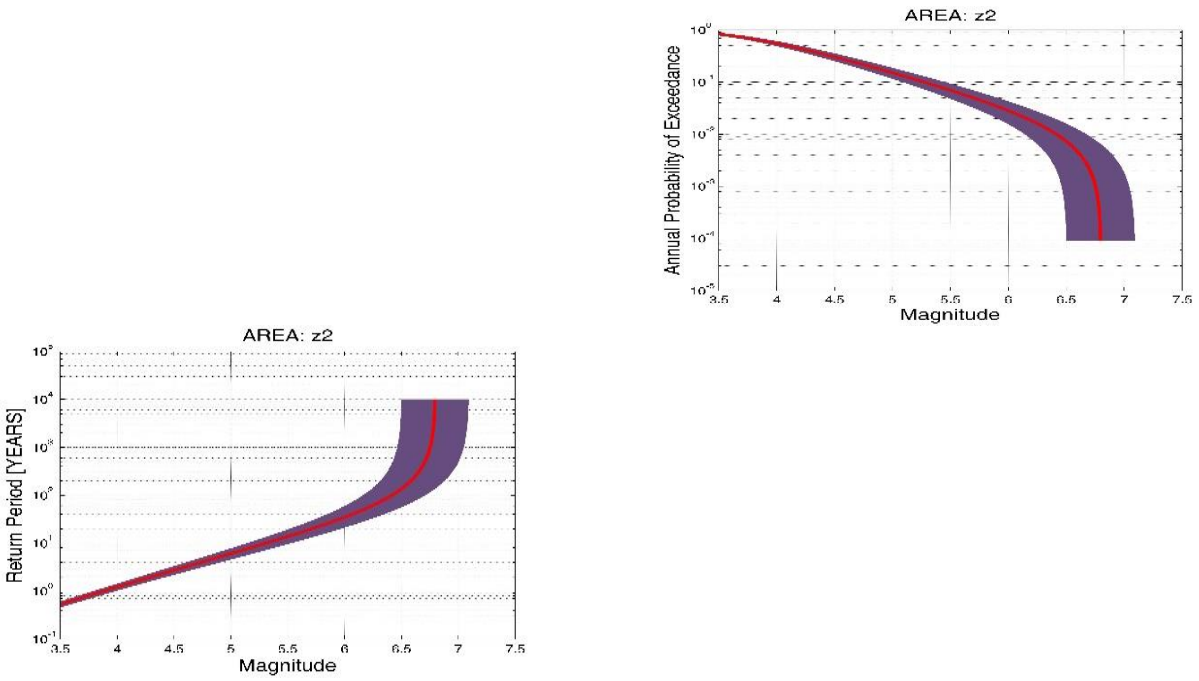
Figure 4. The frequency diagram and return period for Zone 2.
