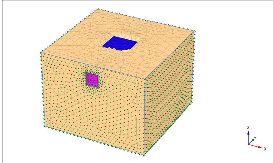
Figure 4. boundary condition
