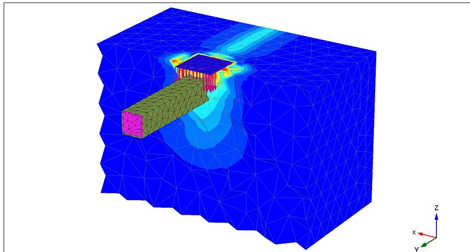
Figure 5. Total displacements |u| (scaled up 5.00 times) Maximum value = 2.740 cm (Element 4918 at Node 3573)
