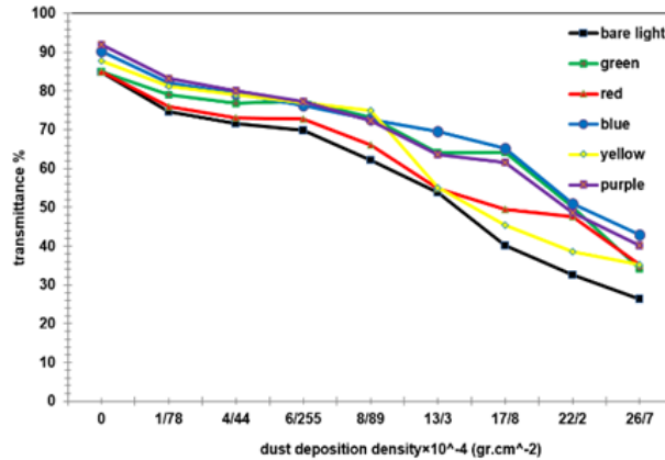
Figure 6 : The transmittance changes of SG windowpanes versus dust settlement density
