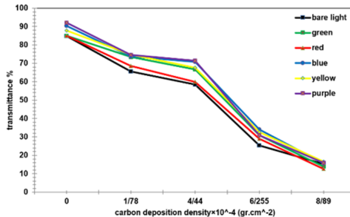
Figure 8. The transmittance changes of SG windowpanes versus dust and carbon mixture settlement density.
