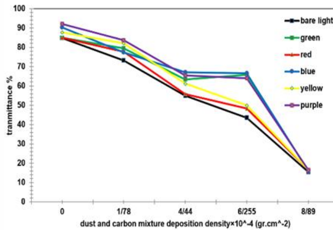
Figure 7. The transmittance changes of SG windowpanes versus carbon settlement density.
