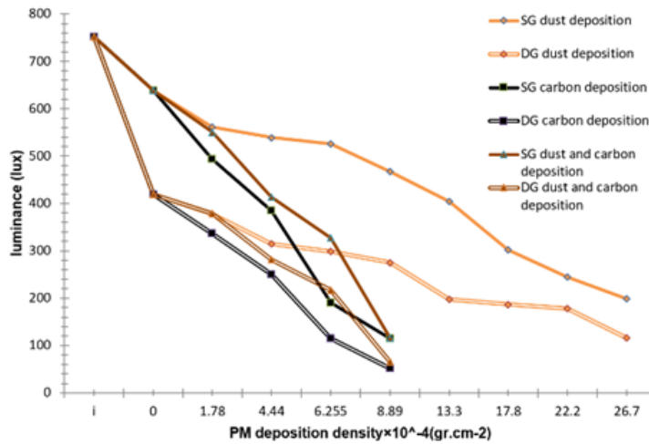
Figure 5. The luminance changes versus dust and pollutant settlement density for SG and DG glaze windowpanes.
