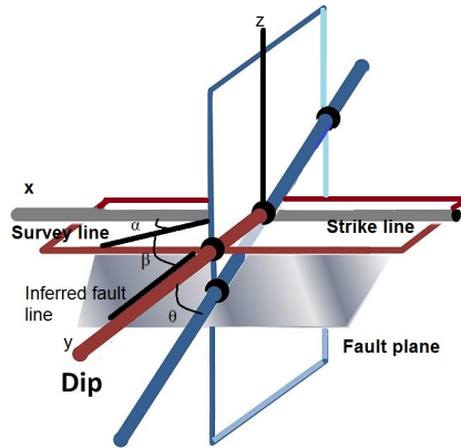
Figure 2: Dip and strike represented by coordinates, \alpha indicates the angle between the survey line and the strike, \beta the angle between the surface and the fault line seen in the tomography, and \theta is the dip angle.
