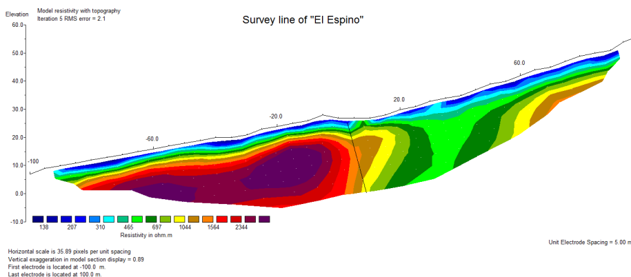
Figure 3: Resistivity profile across the survey line after topography corrections and 5 iterations in the inversion program, for a RMS error of 2.1%. The black line represents the inferred fault. The resistivity values are shown in a logarithmic scale.
